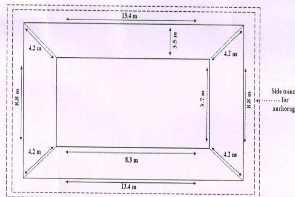
PLAN FOR POND LINING AT PFDC FARM, QUAT, BHUBANESWAR, ODISHA
